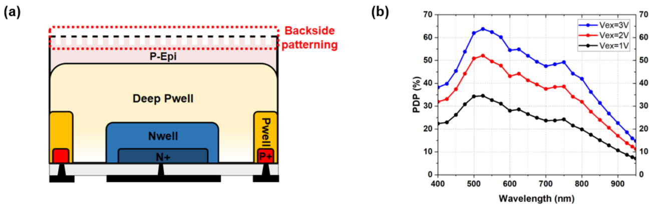
Fig. 1: (a) Cross-section of BI non-isolated SPAD and (b) its PDP performance
